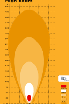
N4701 25200lm High Beam
